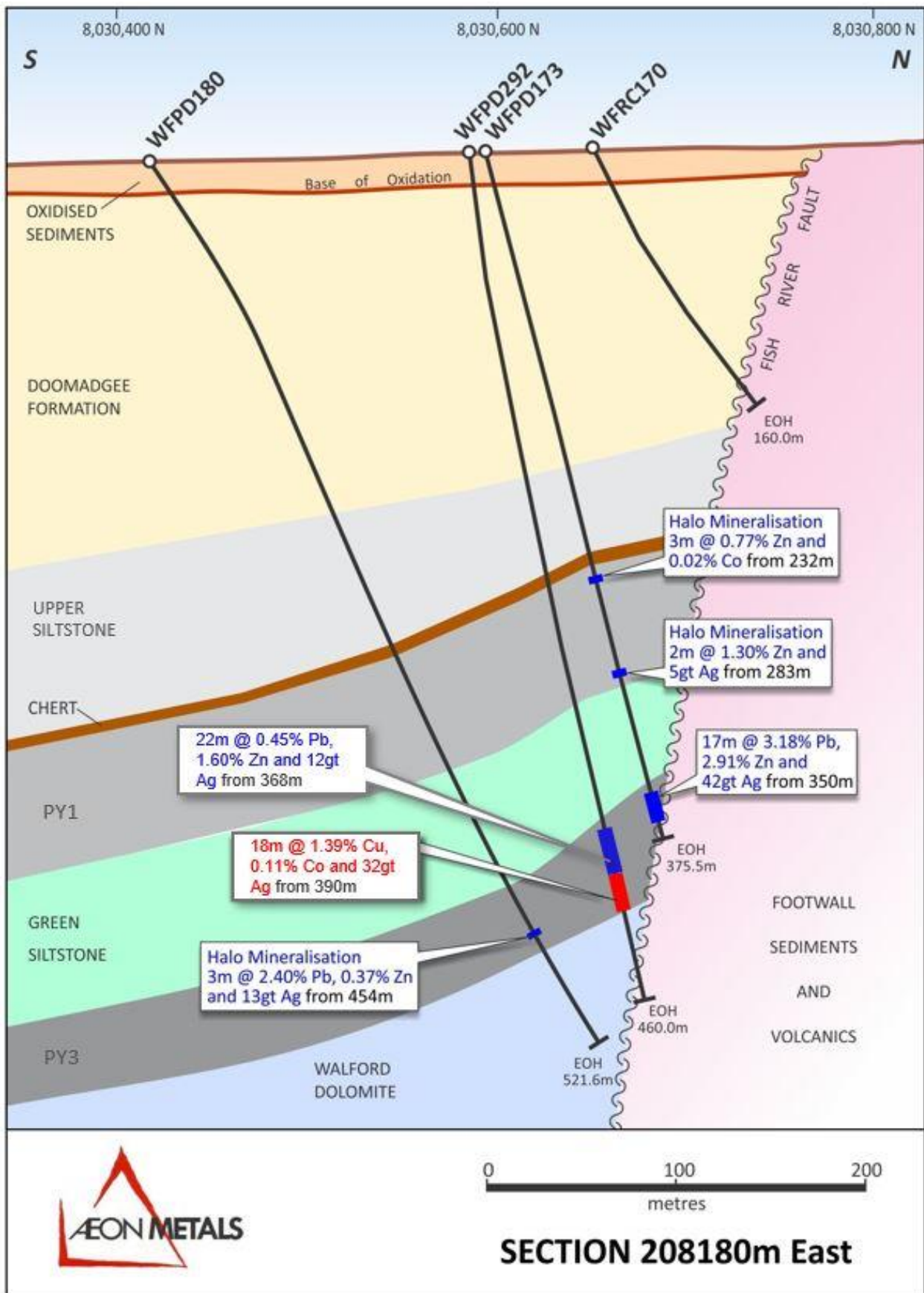
Figure 1 Section 208180E Geological section shows hole WFPD173 and current high grade Copper-Cobalt hole WFPD292
