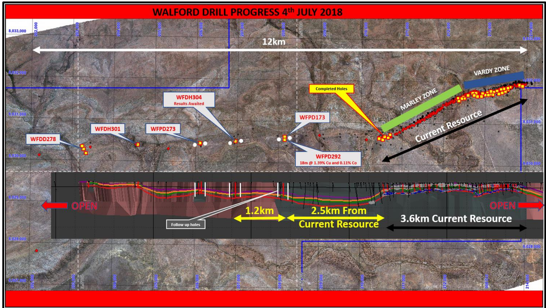
Figure 2 Location of completed holes including extended hole WFPD173 and current hole WFPD292 along strike from the Resource. The plan shows indicative planned holes (red) and the location of the prospective stratigraphy in the Long Section. Hole WFPD304 where a similar zone of chalcopyrite to WFPD292 was intercepted is shown and results are awaited. Proposed follow up holes to the west of the Resource are shown as white traces on the inserted Long Section. These will be drilled approximately 100m either side of those current sections.
