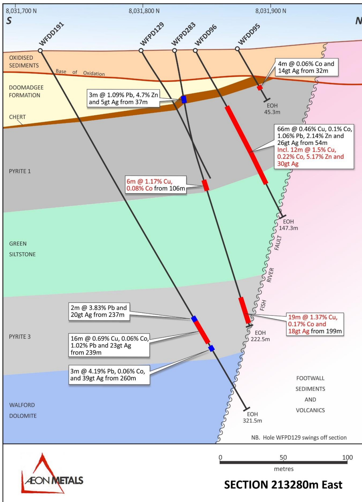
Figure 2: Section showing hole WFPD283 on section 213280E
