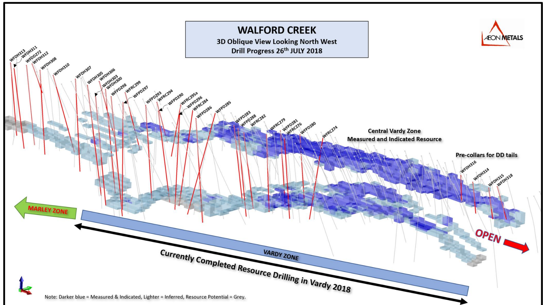
Figure 6: Vardy Resource drilling.
