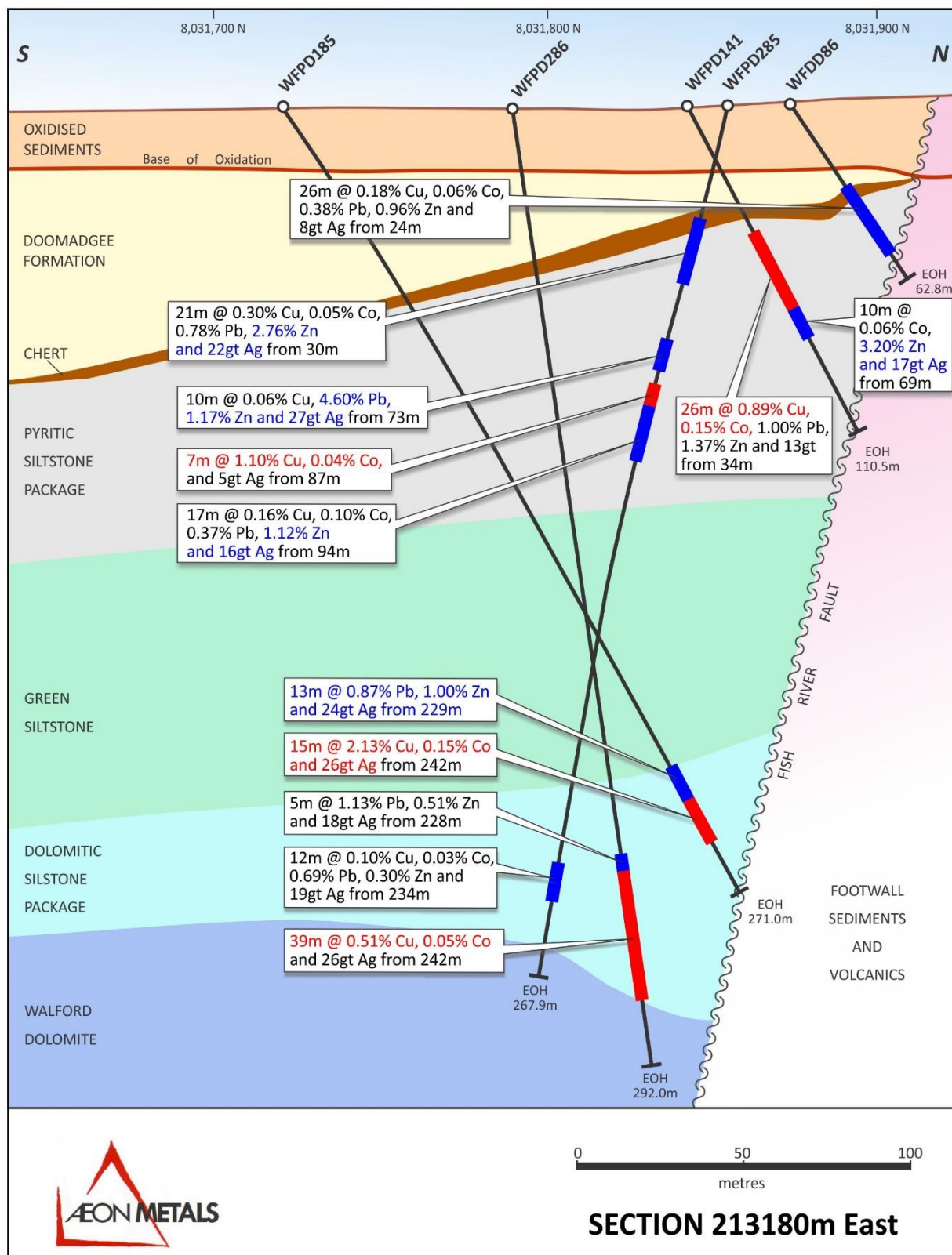
Figure 3: Section showing holes WFPD285 and 286 on section 213180E
