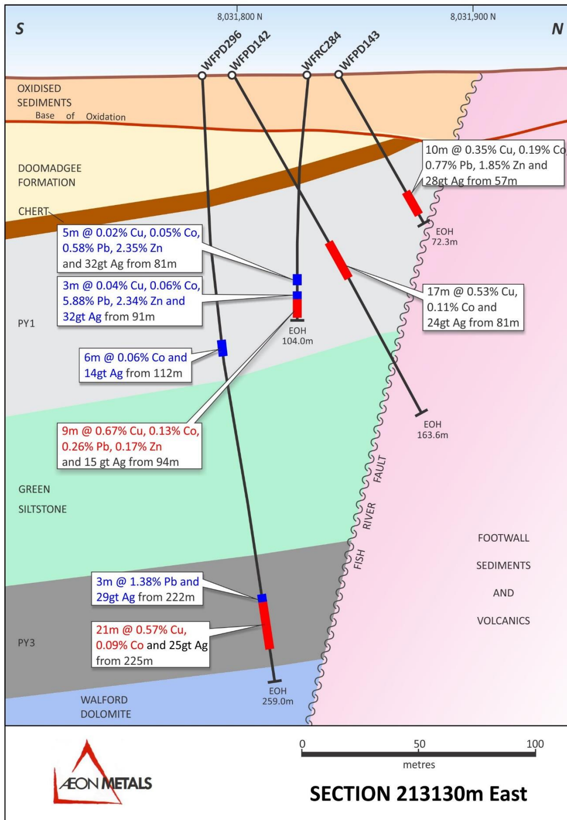
Figure 4: Section showing holes WFR284 and WFPD296 on section 213130E
