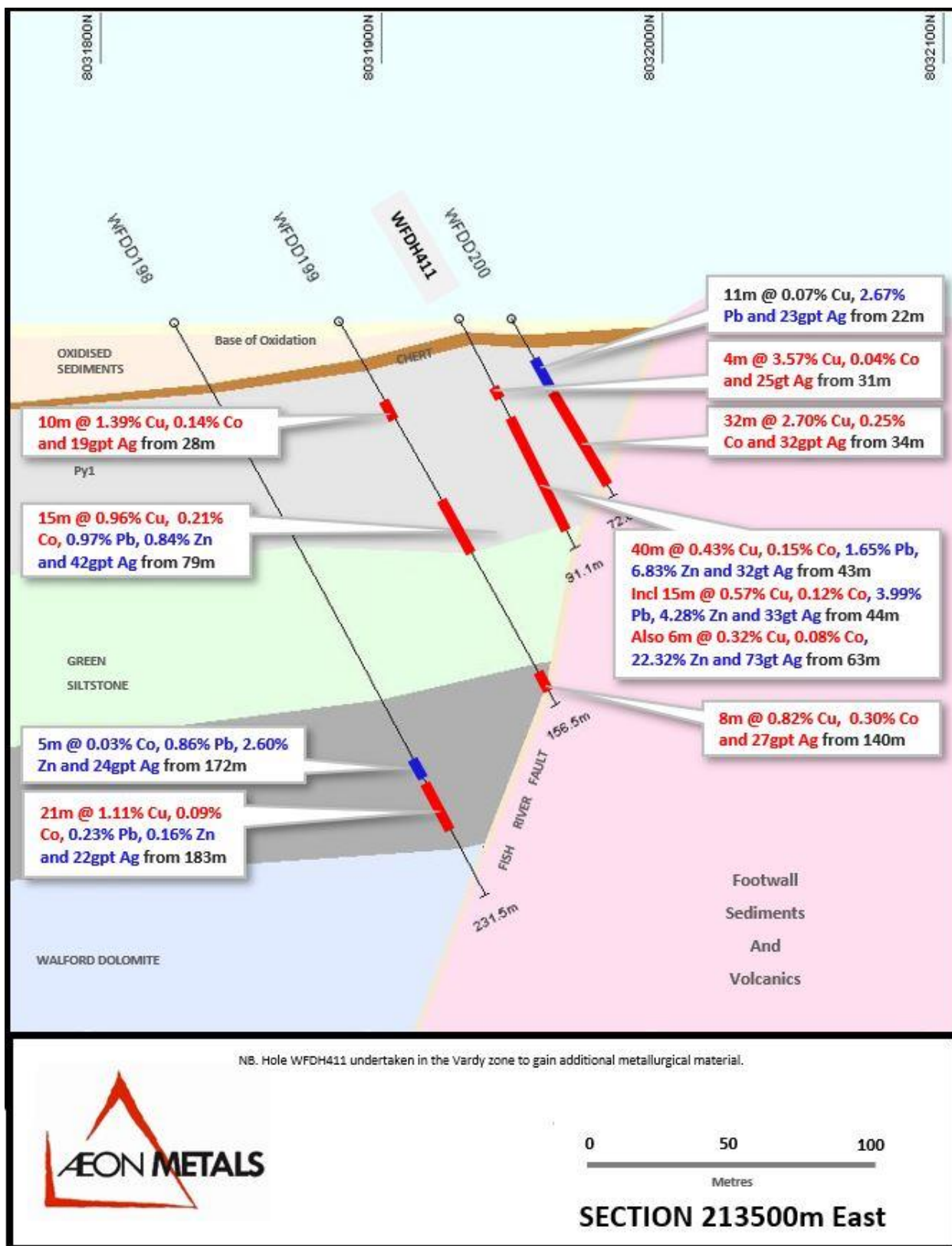
Figure 22: Section 213500E showing hole WFDH411
