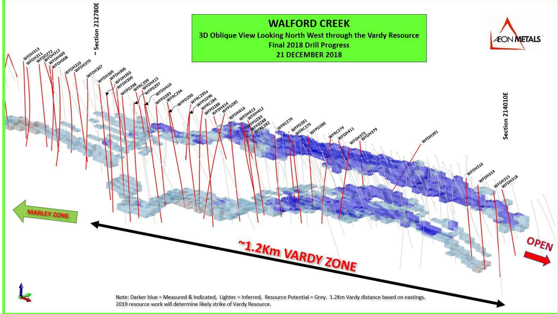
Figure 6. Oblique view of the Vardy drilling with all holes completed in 2018.
