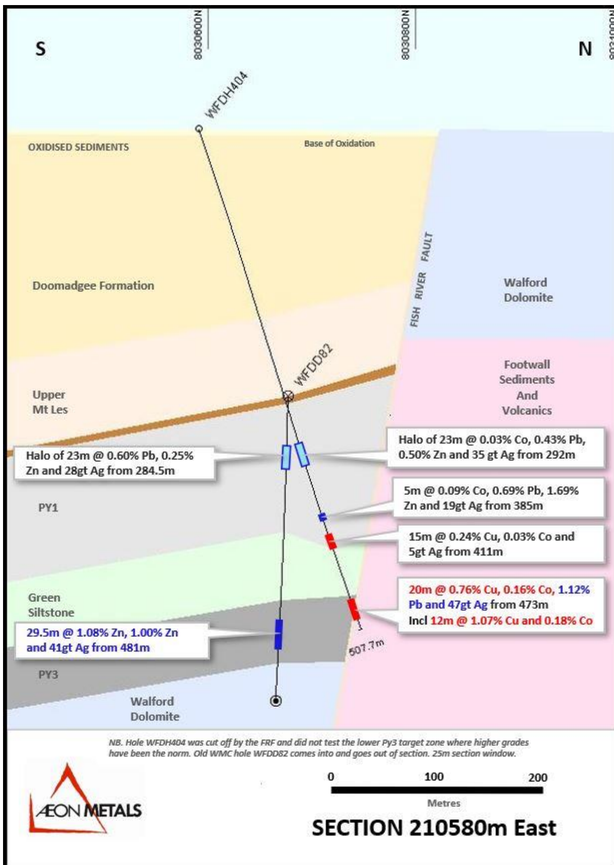
Figure 7: Section 210580E showing recent hole WFDH404
