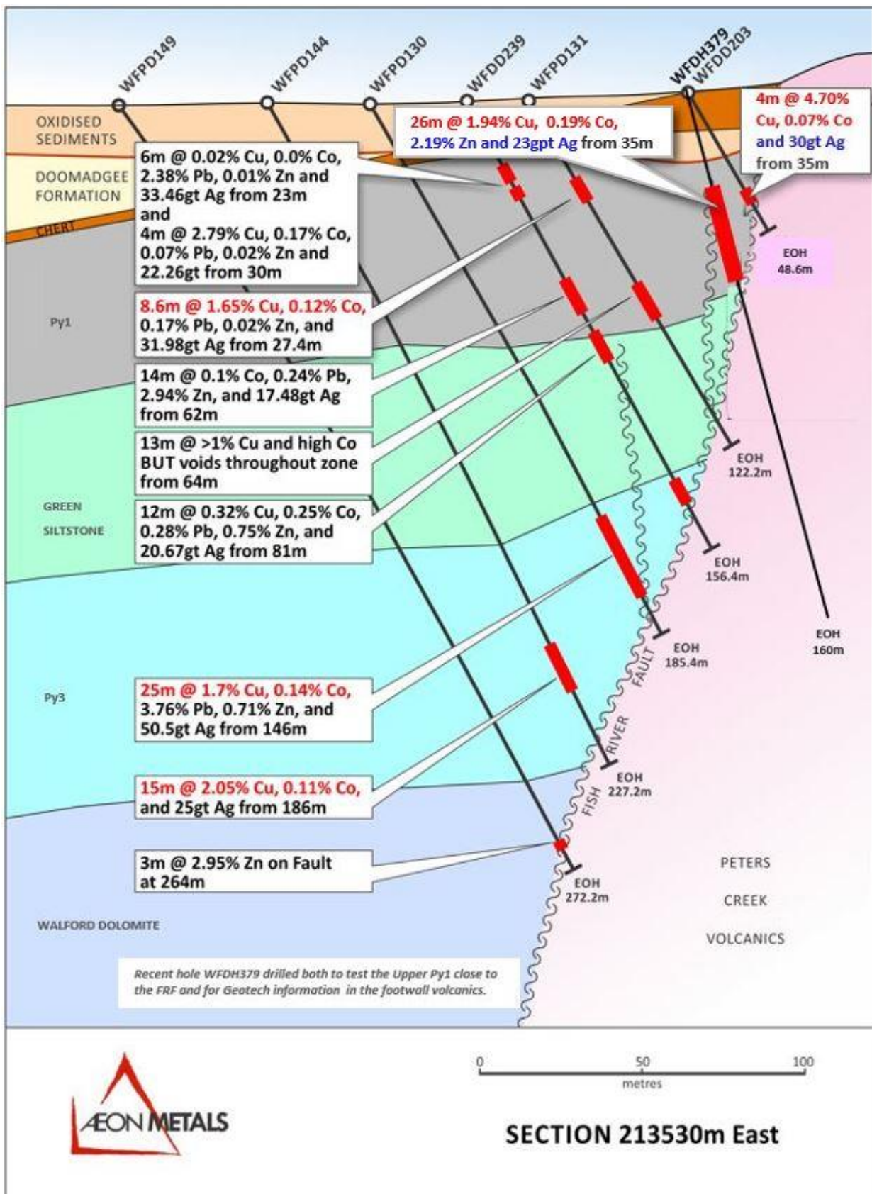
Figure 23: Section 213530E showing hole WFDH379
