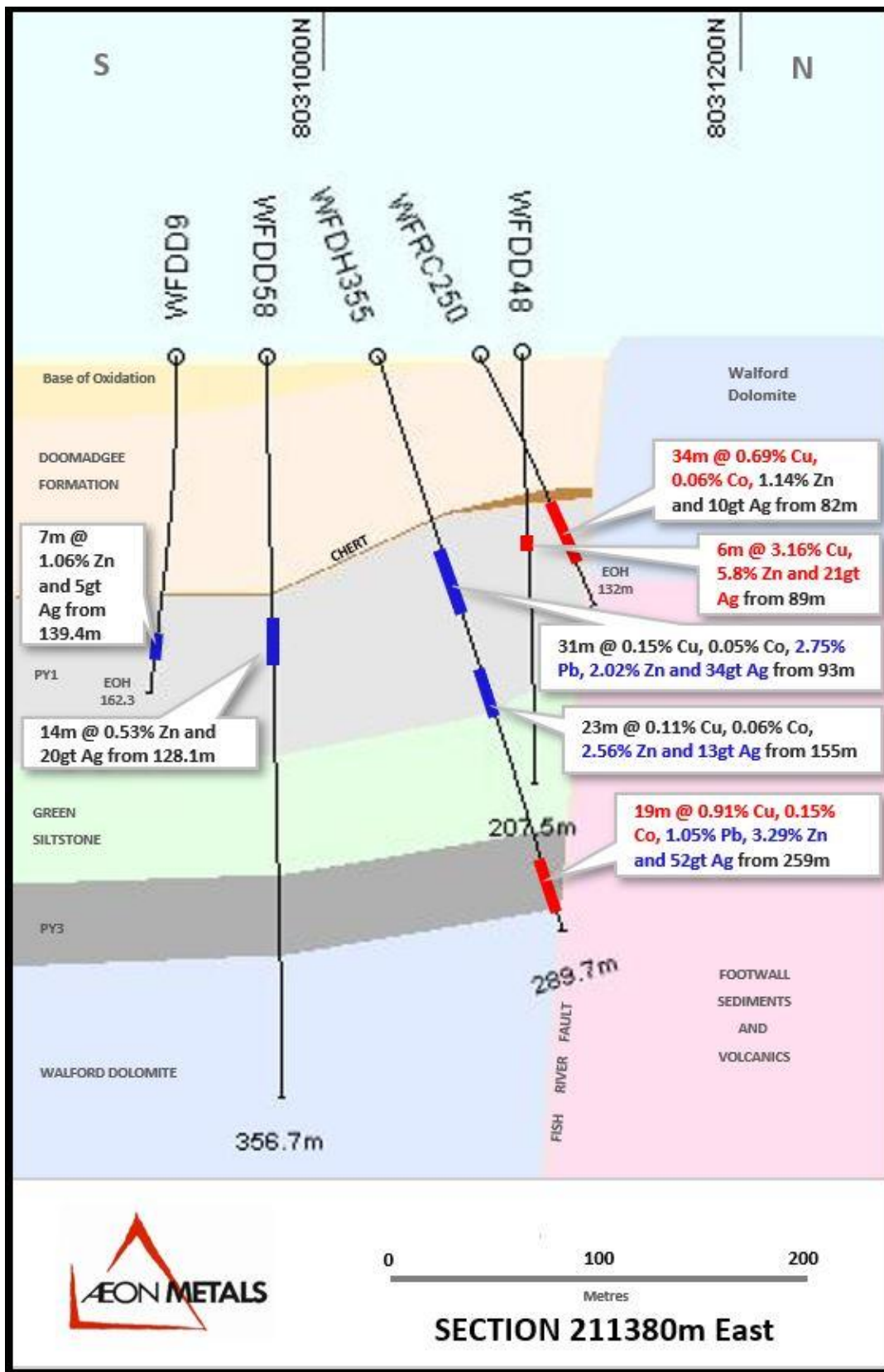
Figure 12: Section 211380E showing hole WFDH355
