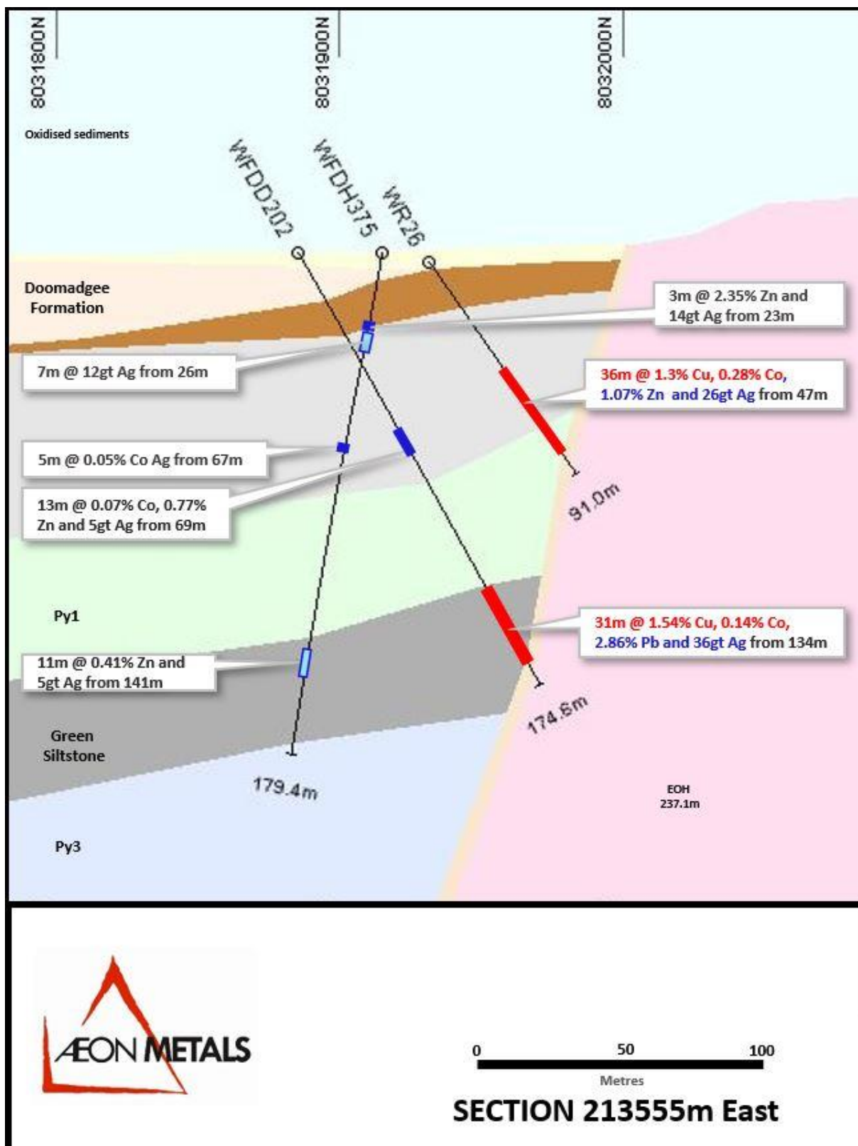
Figure 24: Section 213555E showing hole WFDH375
