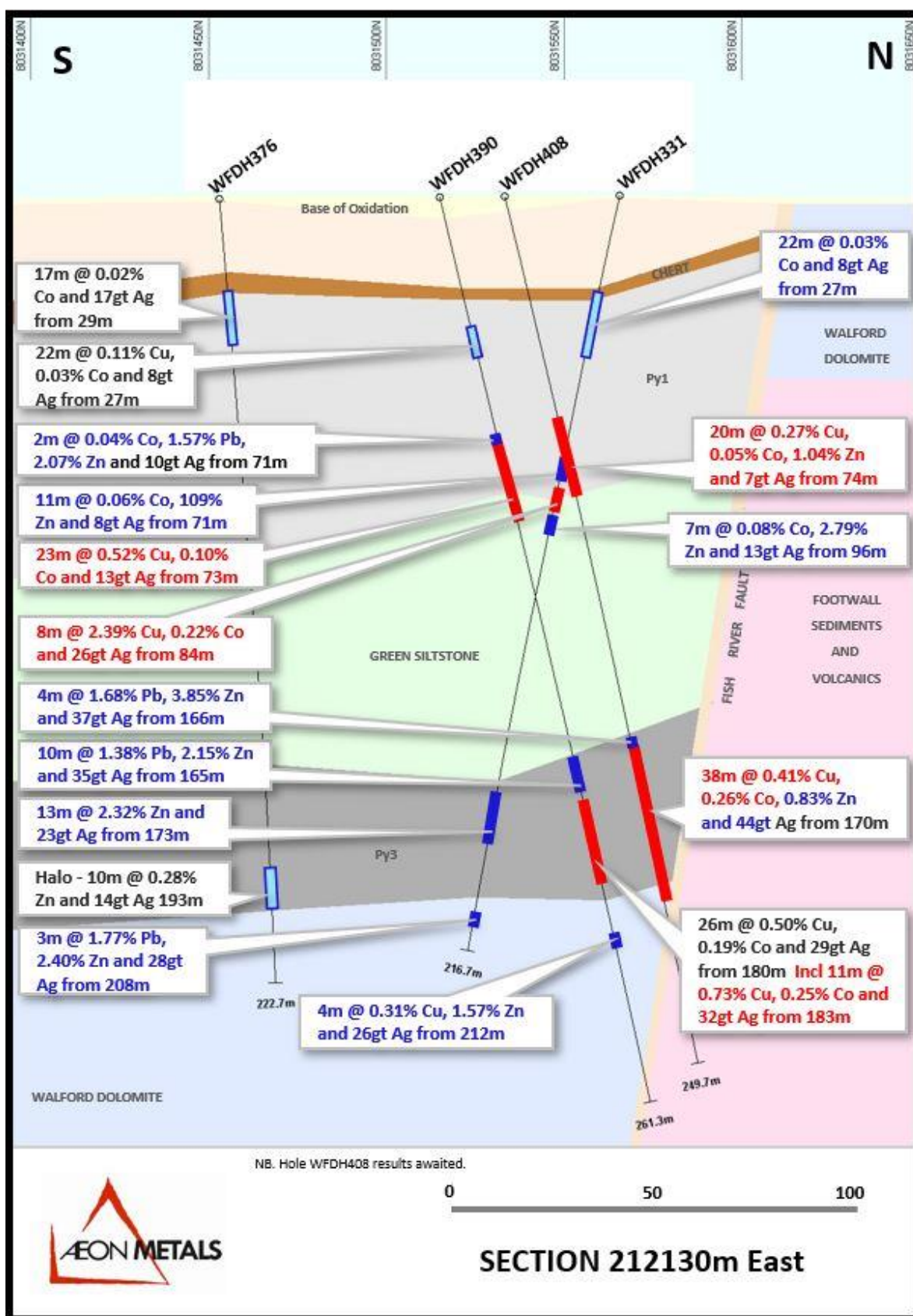
Figure 15: Section 212130E showing WFDH408
