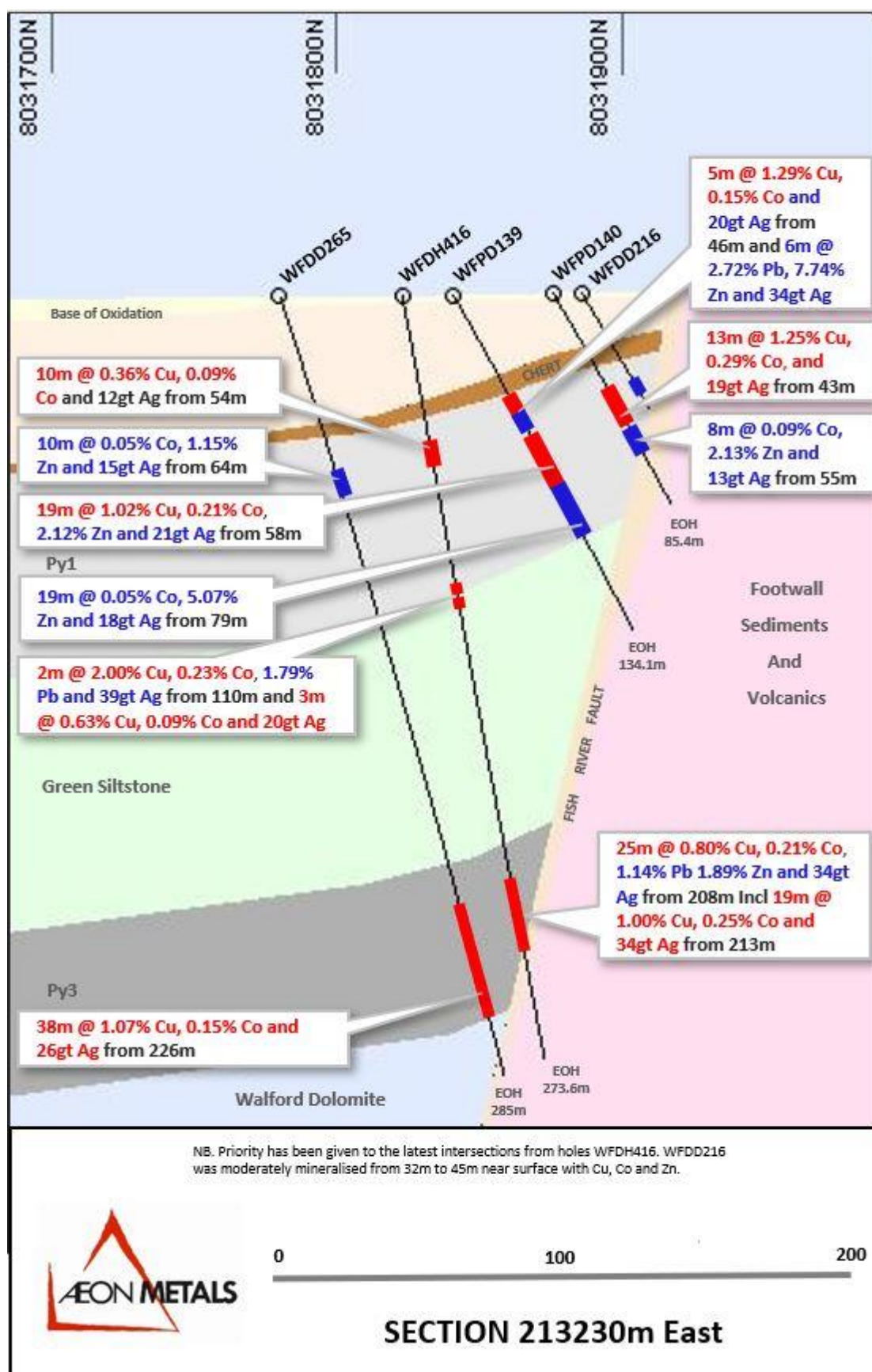
Figure 20: Section 213230E showing hole WFDH416
