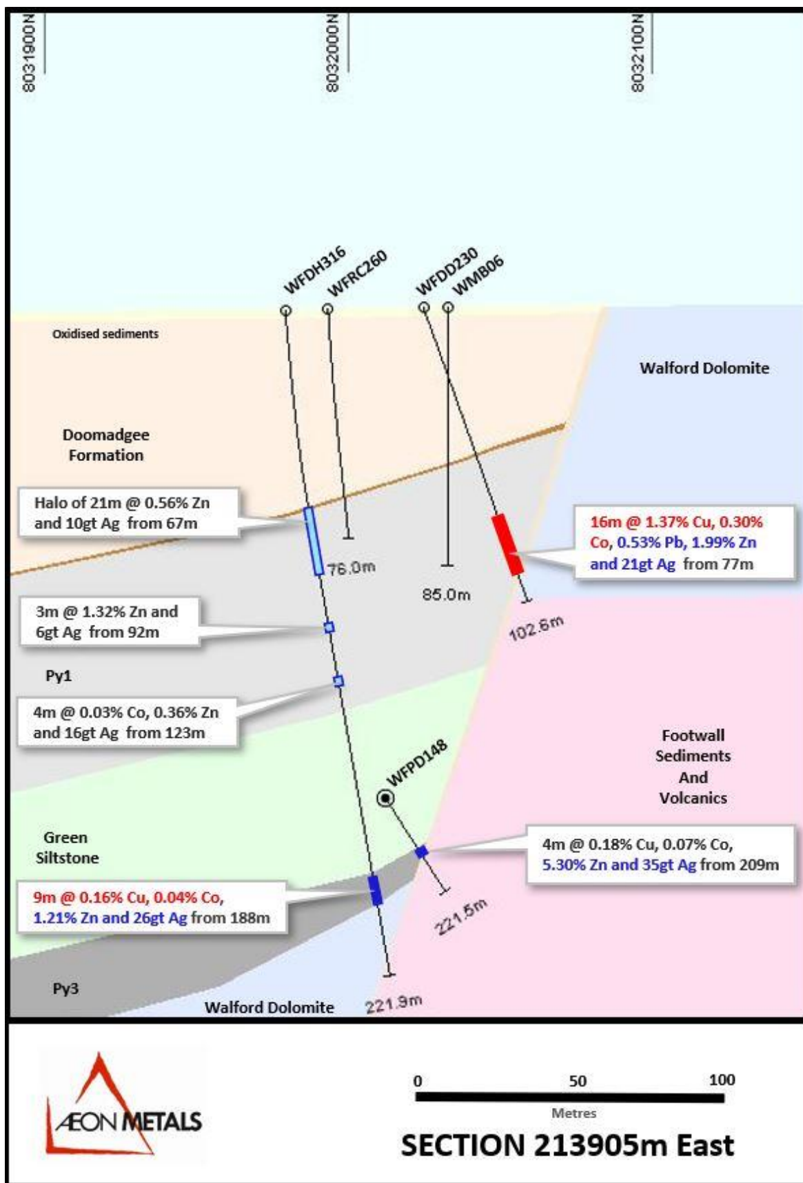
Figure 25: Section 213905E showing hole WFDH316
