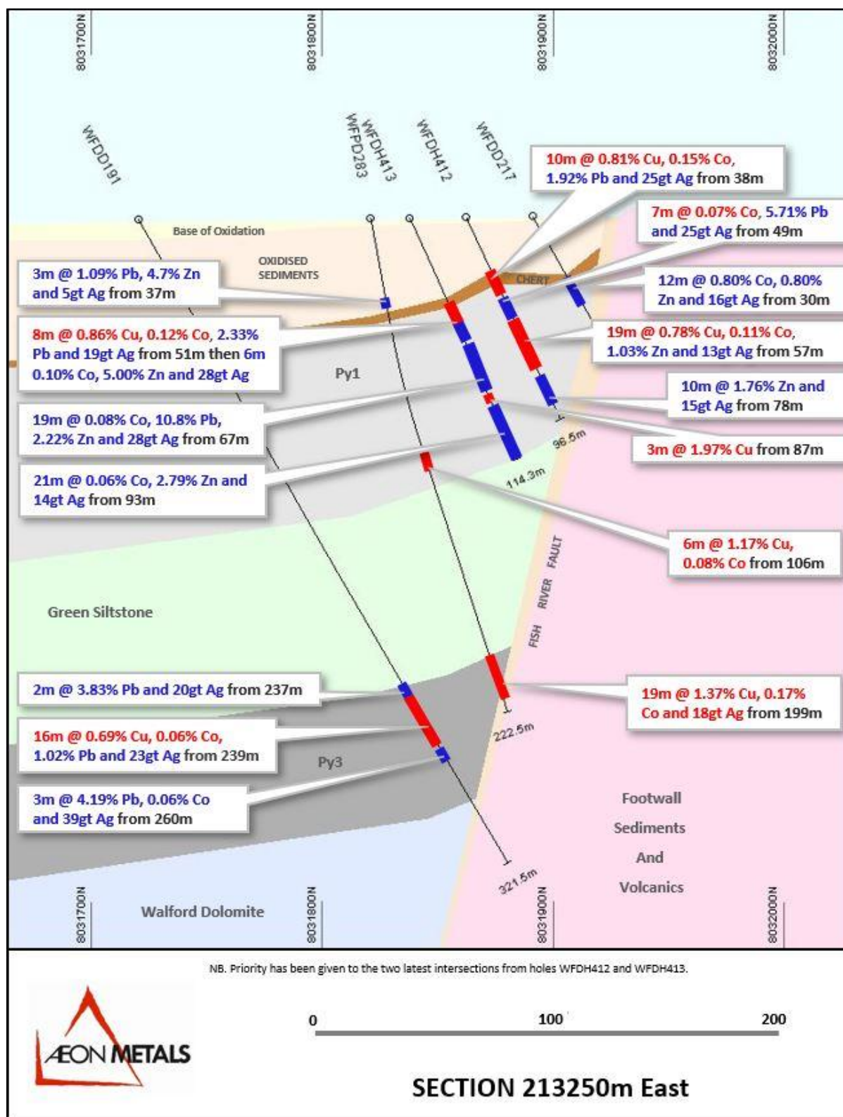
Figure 21: Section 213250E showing holes WFDH412 and WFDH413
