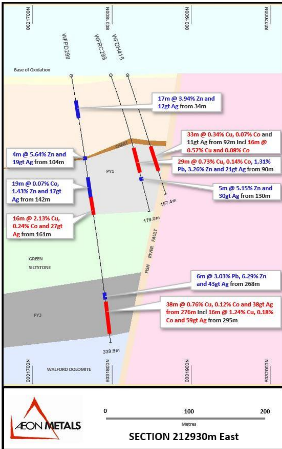
Figure 17: Section 212930E showing hole WFDH415
