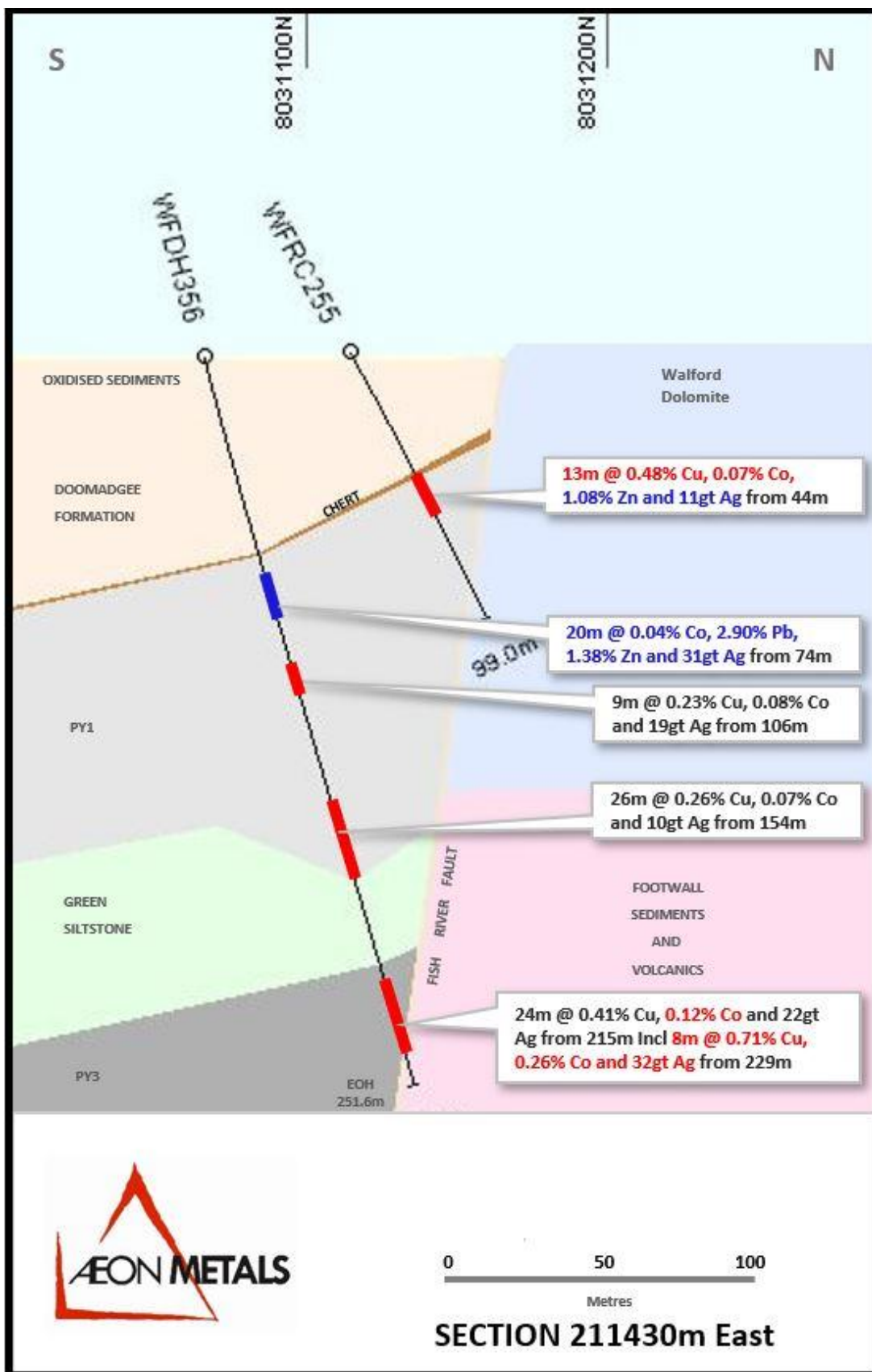
Figure 13: Section 211430E showing hole WFDH356
