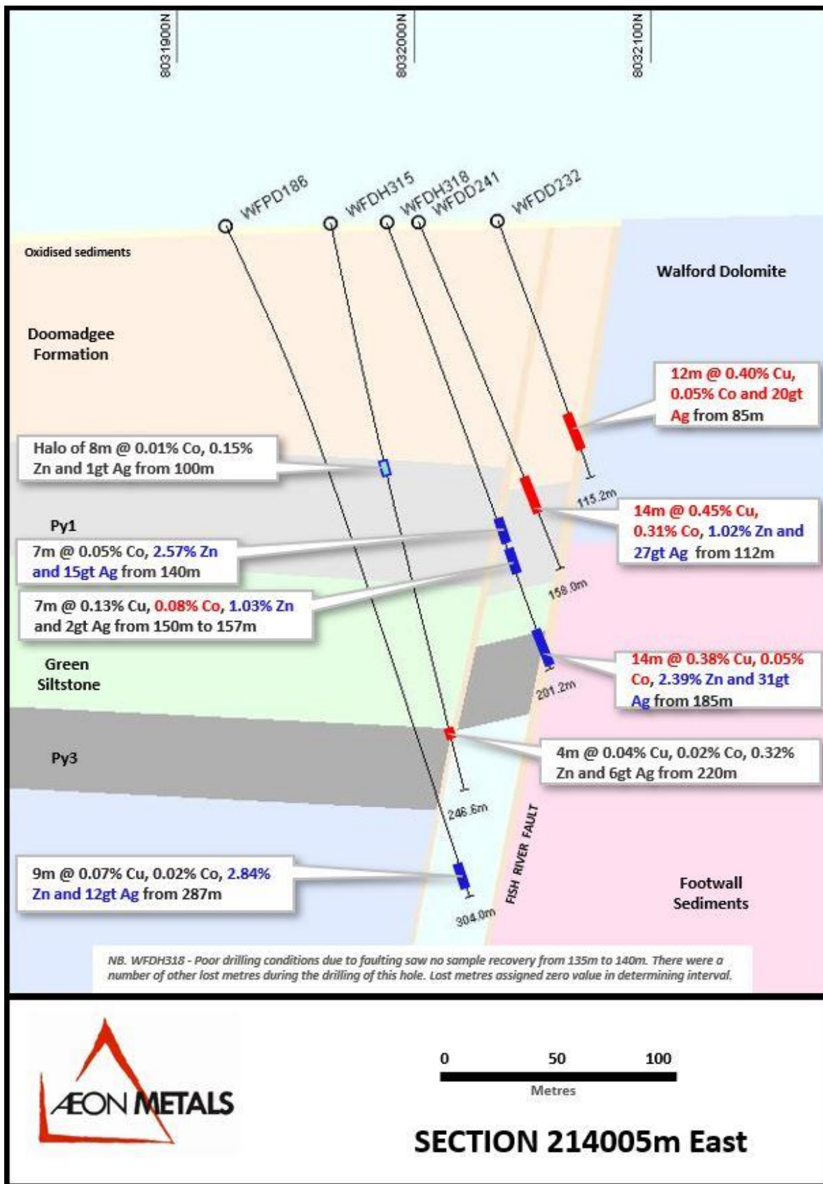
Figure 27: Section 214005E showing hole WFDH315 and WFDH318
