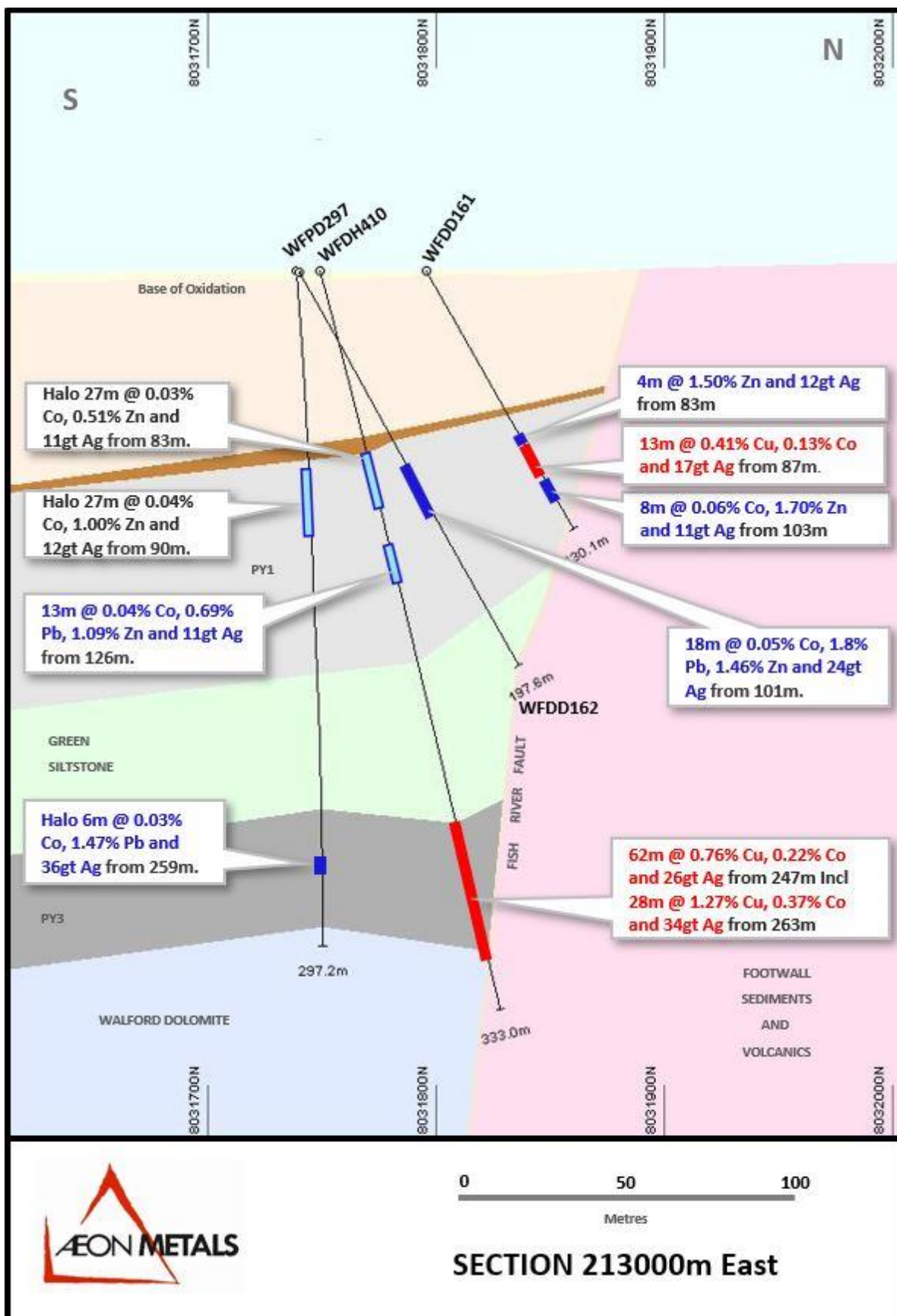
Figure 18: Section 213000E showing hole WFDH410
