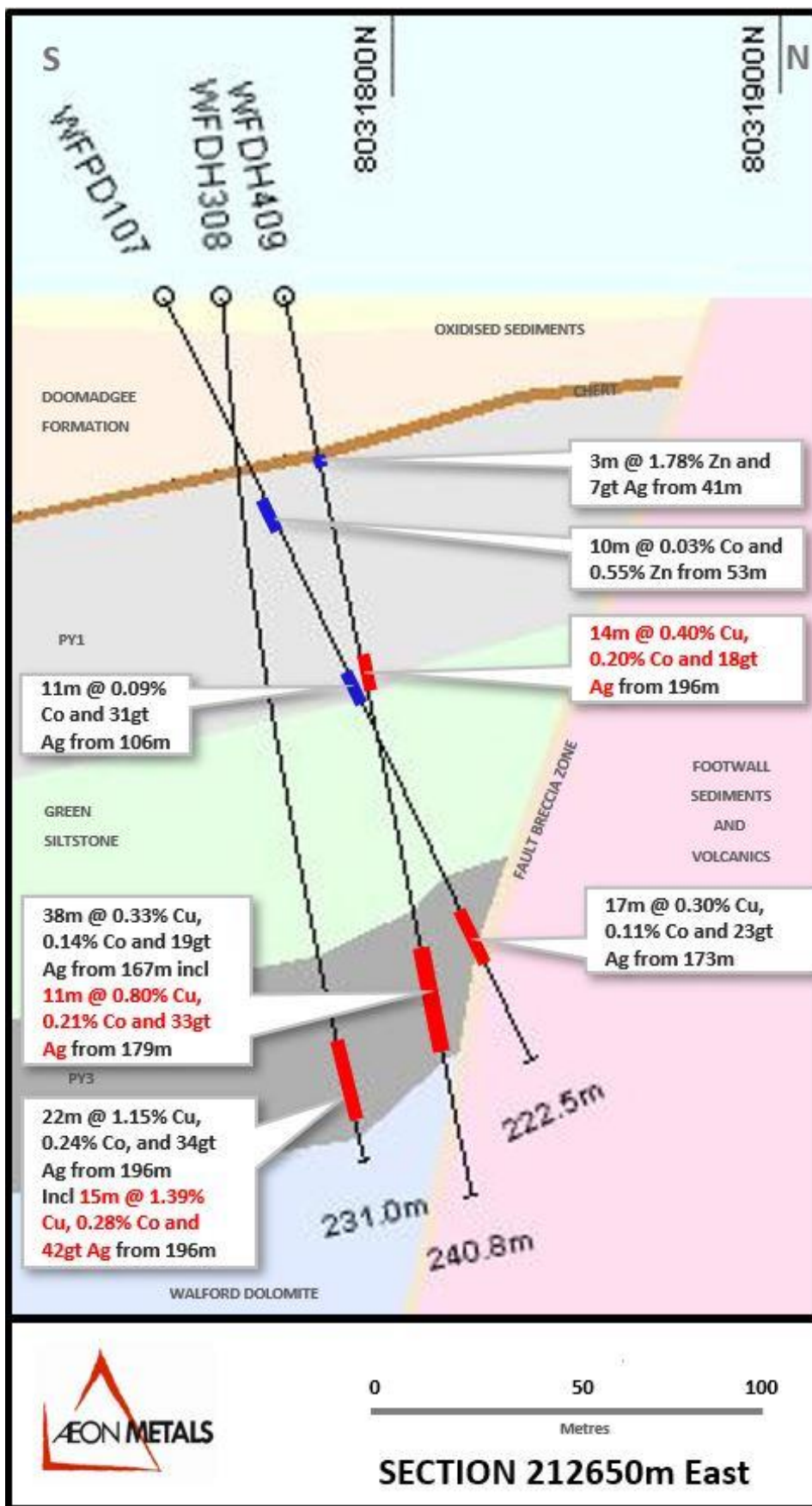
Figure 16: Section 212650E showing old hole WFDH308 and recent hole WFDH409
