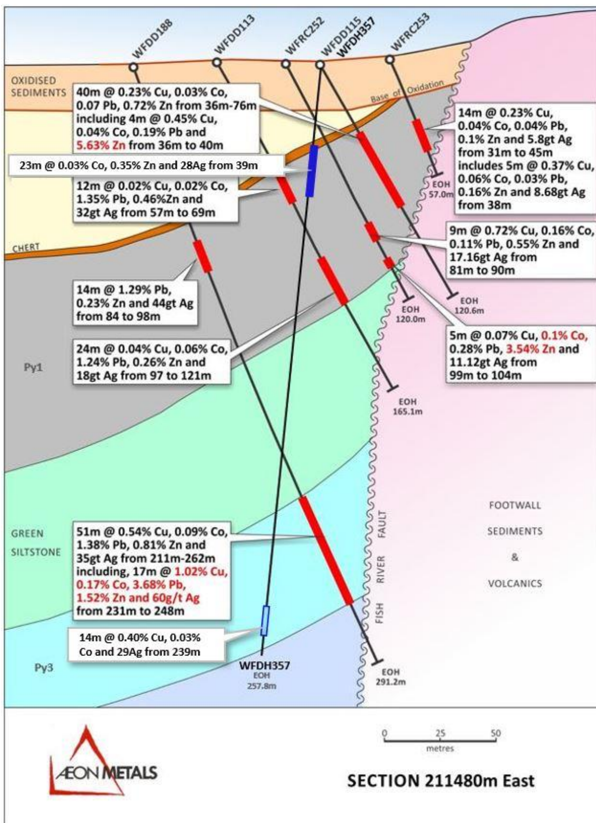
Figure 14: Section 211480E showing hole WFDH357 drilled as a 'close off' hole.
