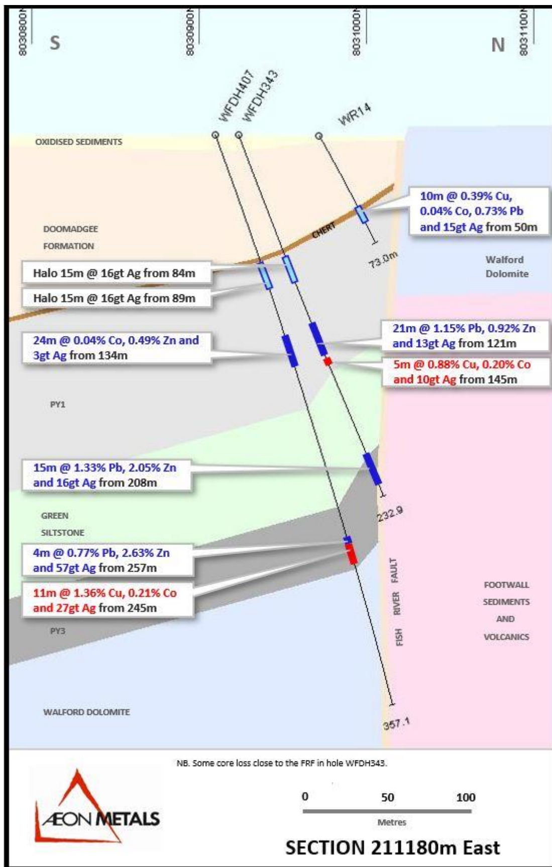
Figure 9: Section 211180E showing hole WFDH407
