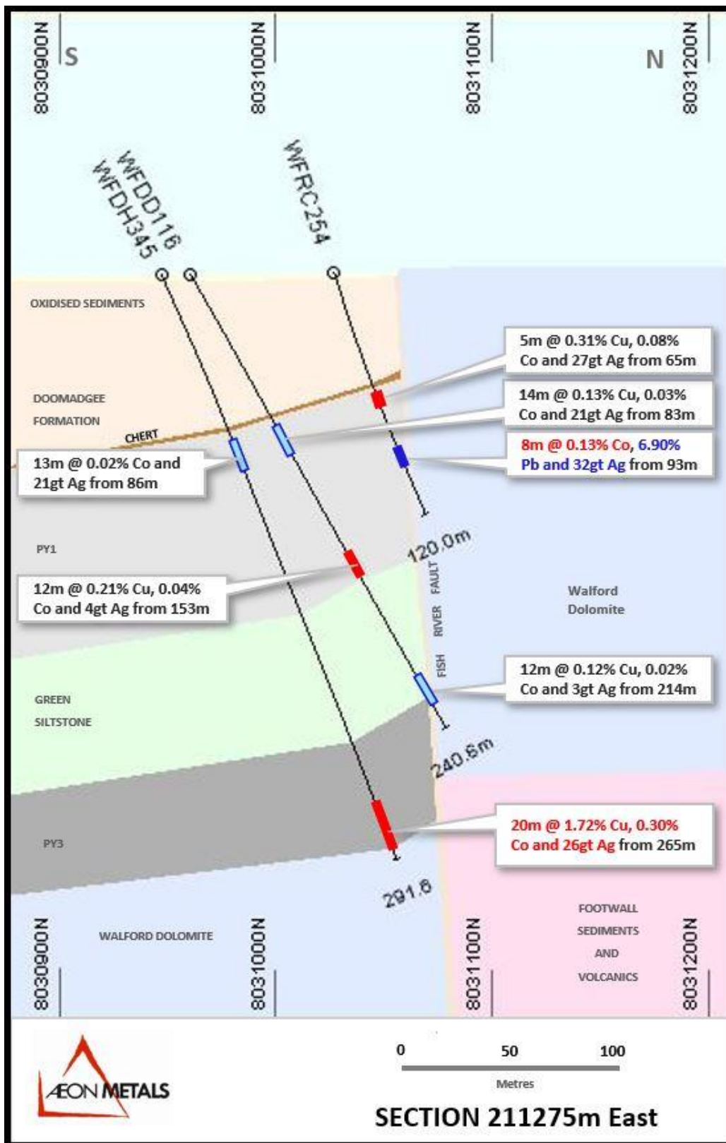
Figure 10: Section 211275EE showing hole WFDH345
