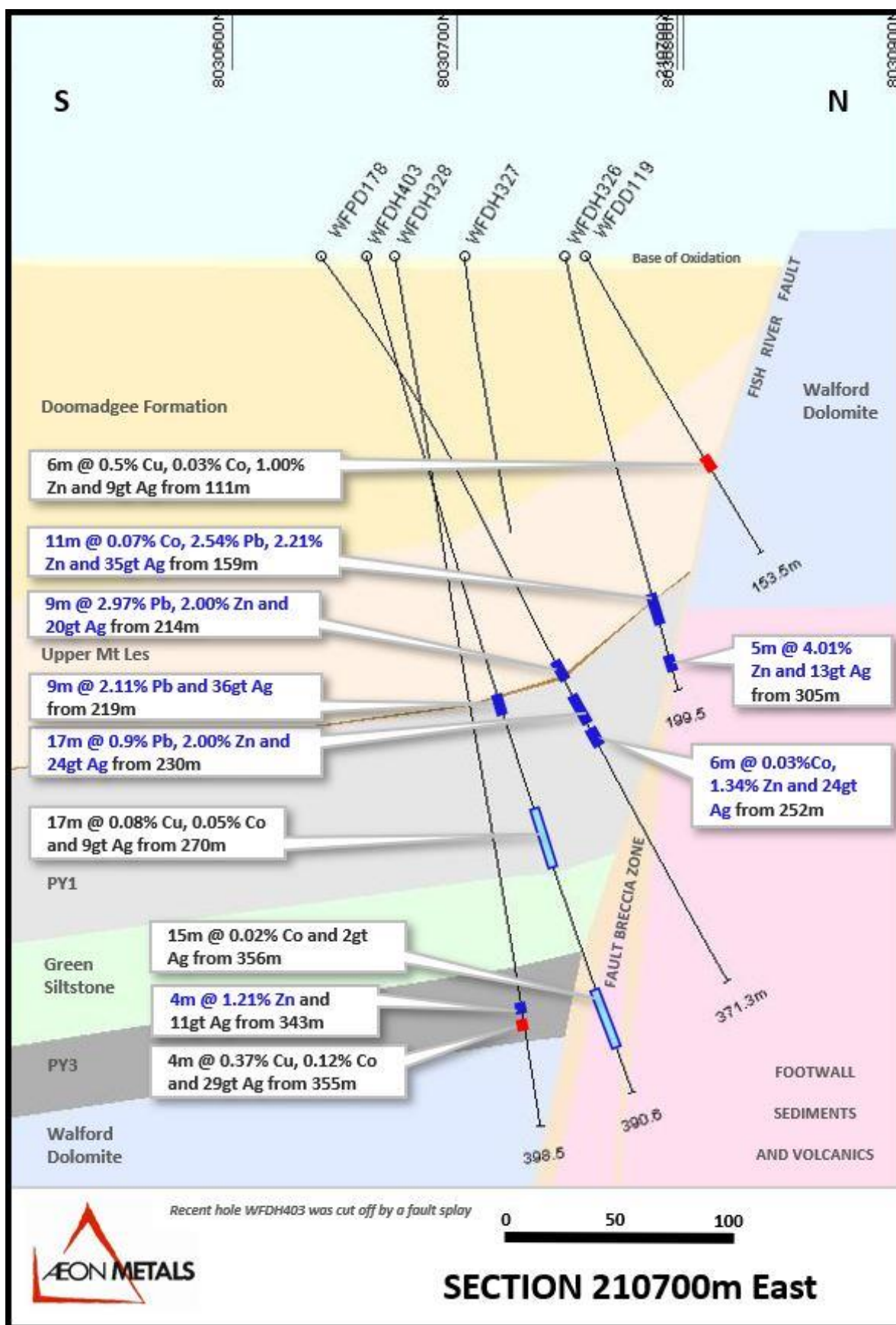
Figure 8: Section 210700E showing recent hole WFDH403 which was cut off by a splay fault off the FRF.
