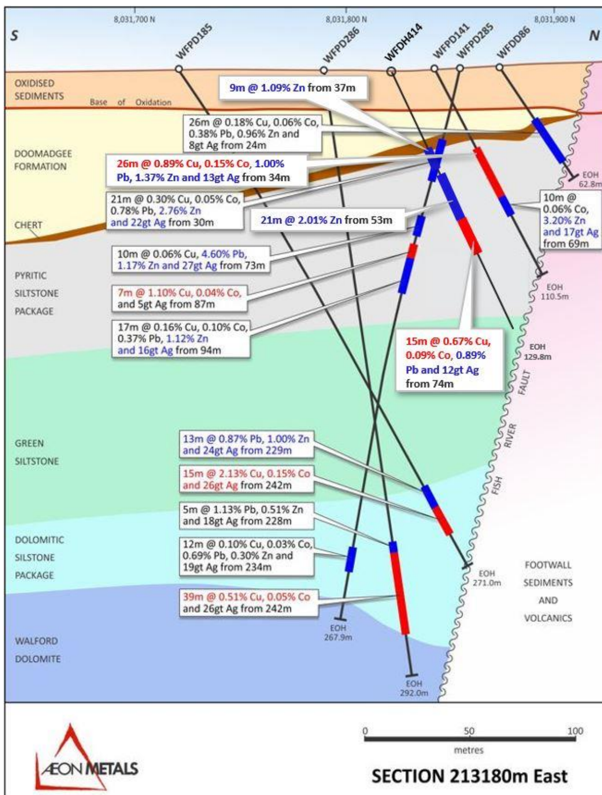
Figure 19: Section 213180E showing hole WFDH414
