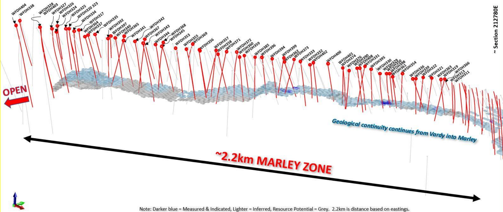
Figure 4. Oblique view of Marley drilling with all holes completed in 2018.
