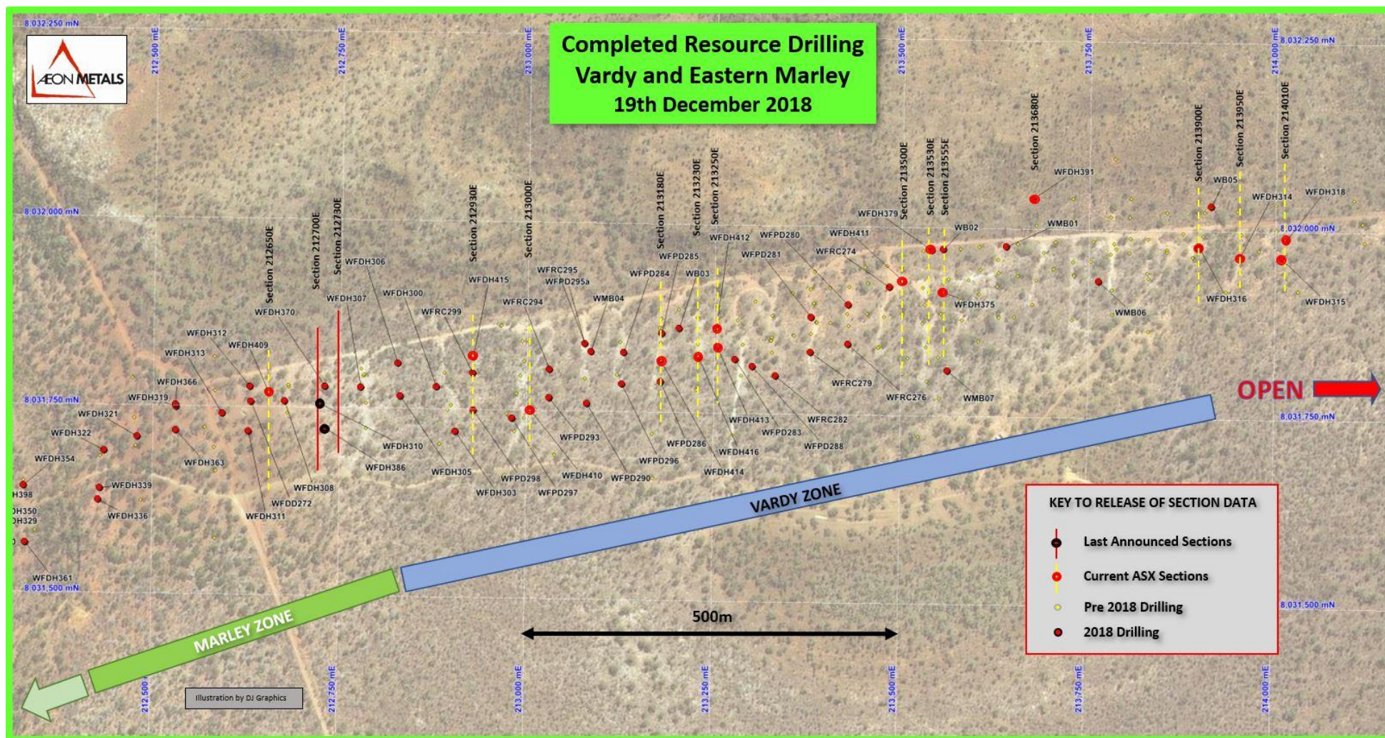
Figure 5: Plan of the Vardy and Eastern Marley drilling showing all holes released previously and in the current ASX announcement.
