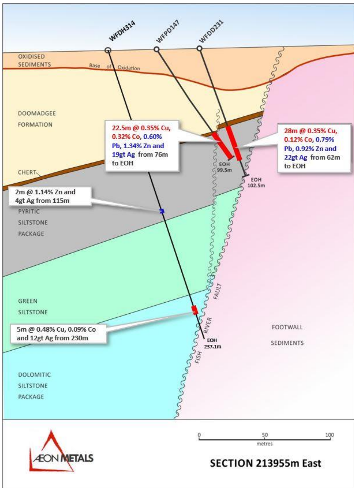
Figure 26: Section 213955E showing WFDH314
