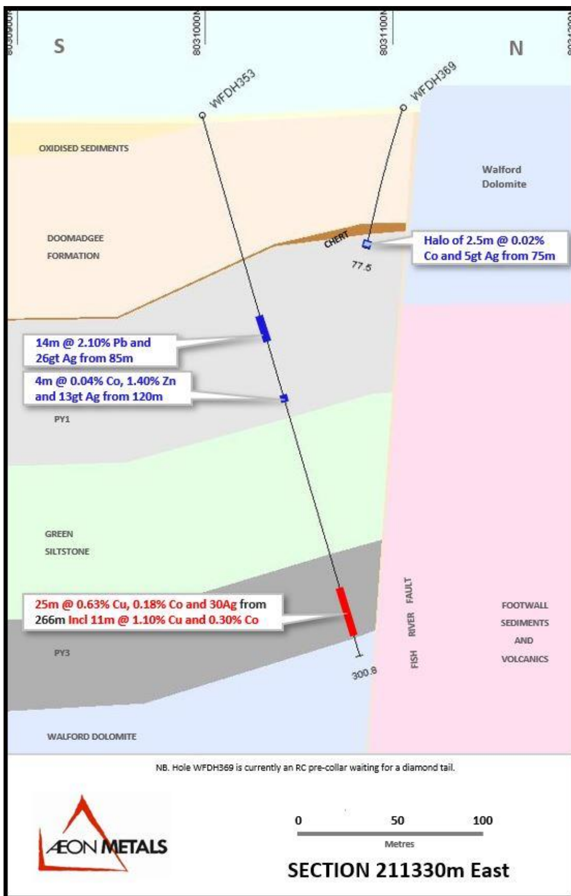
Figure 11: Section 211330E showing completed hole WFDH353 and pre-collar hole WFDH369
