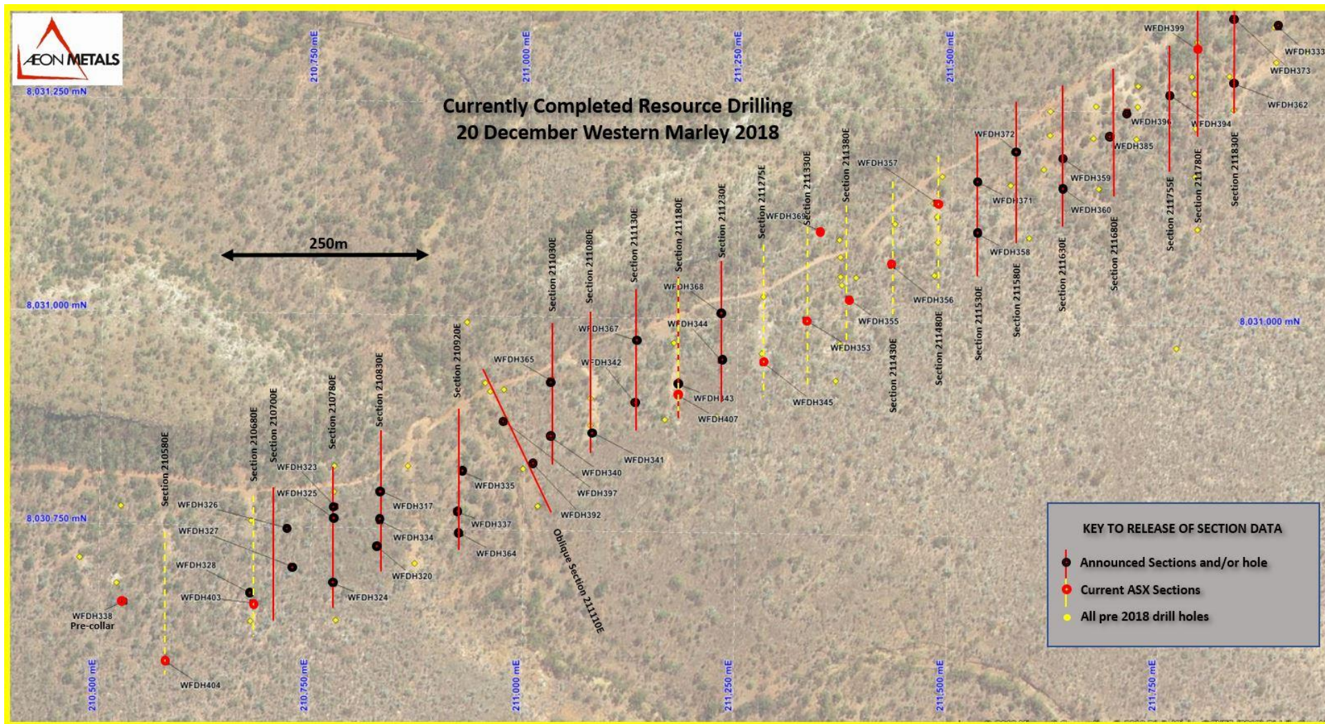
Figure 2: Plan of the Western Marley completed drilling with holes being released for this current ASX release.
