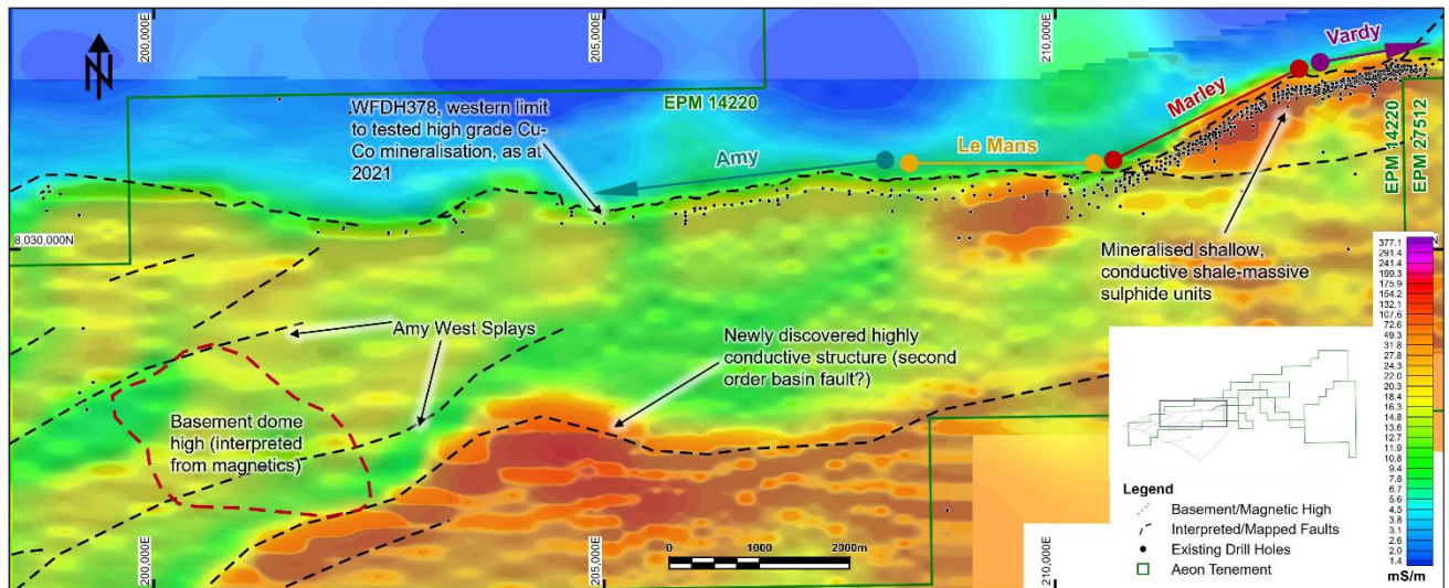
Figure 1. Conductivity over the main Walford Creek mineralised zone
